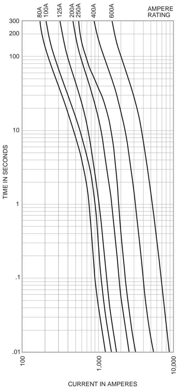
Time-Current Characteristic Curves—Average Melt
