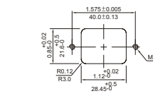
SUGGESTED MOUNTING CUTOUT (MOUNTING FROM FRONT)
