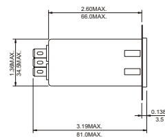
ALL WIRE LEADS 4.0" LONG MIN.
