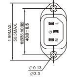
SUGGESTED MOUNTING CUTOUT (MOUNTING FROM FRONT)
